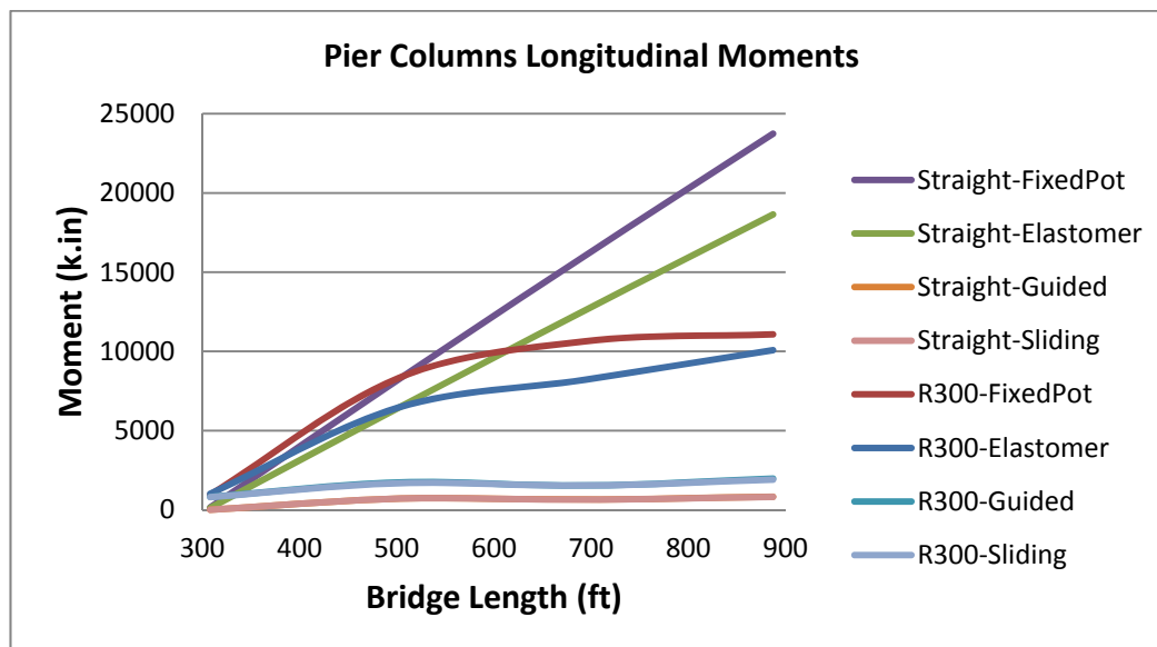
Figure 4.4-43. Longitudinal Bending Moment of Pier Columns with Different Bearing
