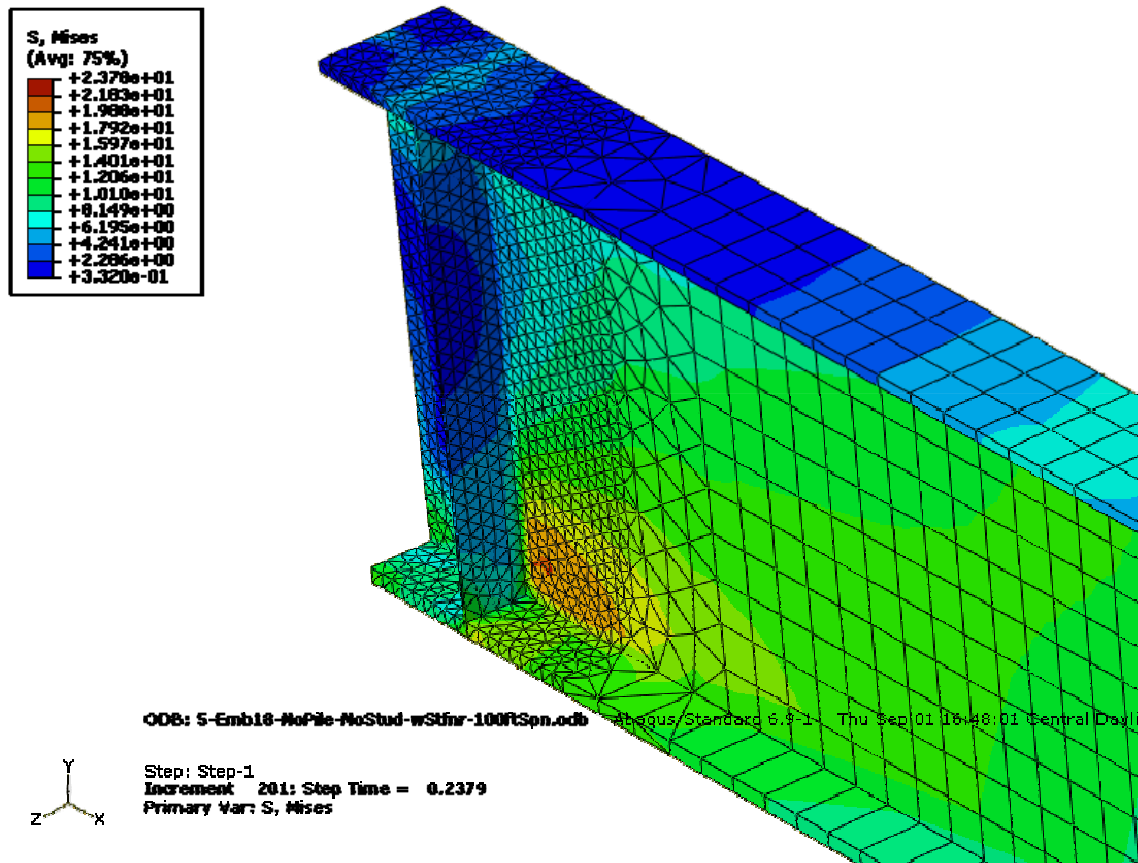
Figure 3.9-2. Mises Stresses of Girder with Stiffener without End Shear Stud
