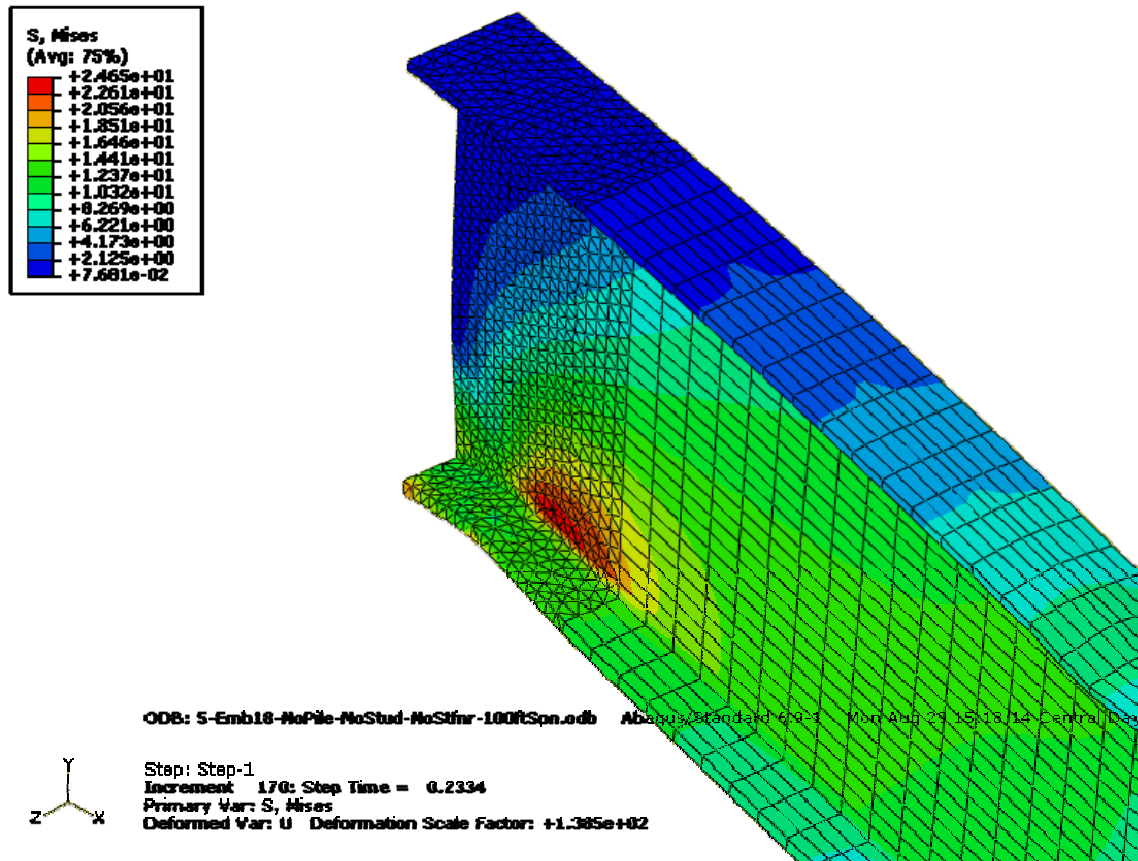
Figure 3.9-1. Mises Stresses of Girder without any Stiffener or End Shear Stud
